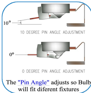
G4-SP - Side View
